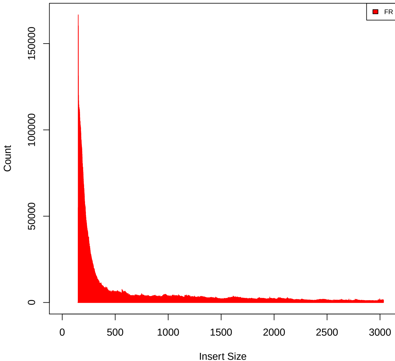
Insert Size Histogram for All_Reads in file G168_G169_M11_primary_unique.bam
