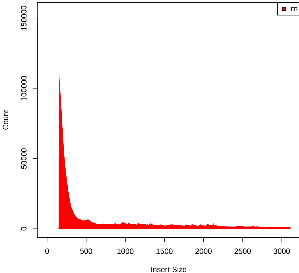
Insert Size Histogram for All_Reads in file G168_G169_M14_primary_unique.bam
