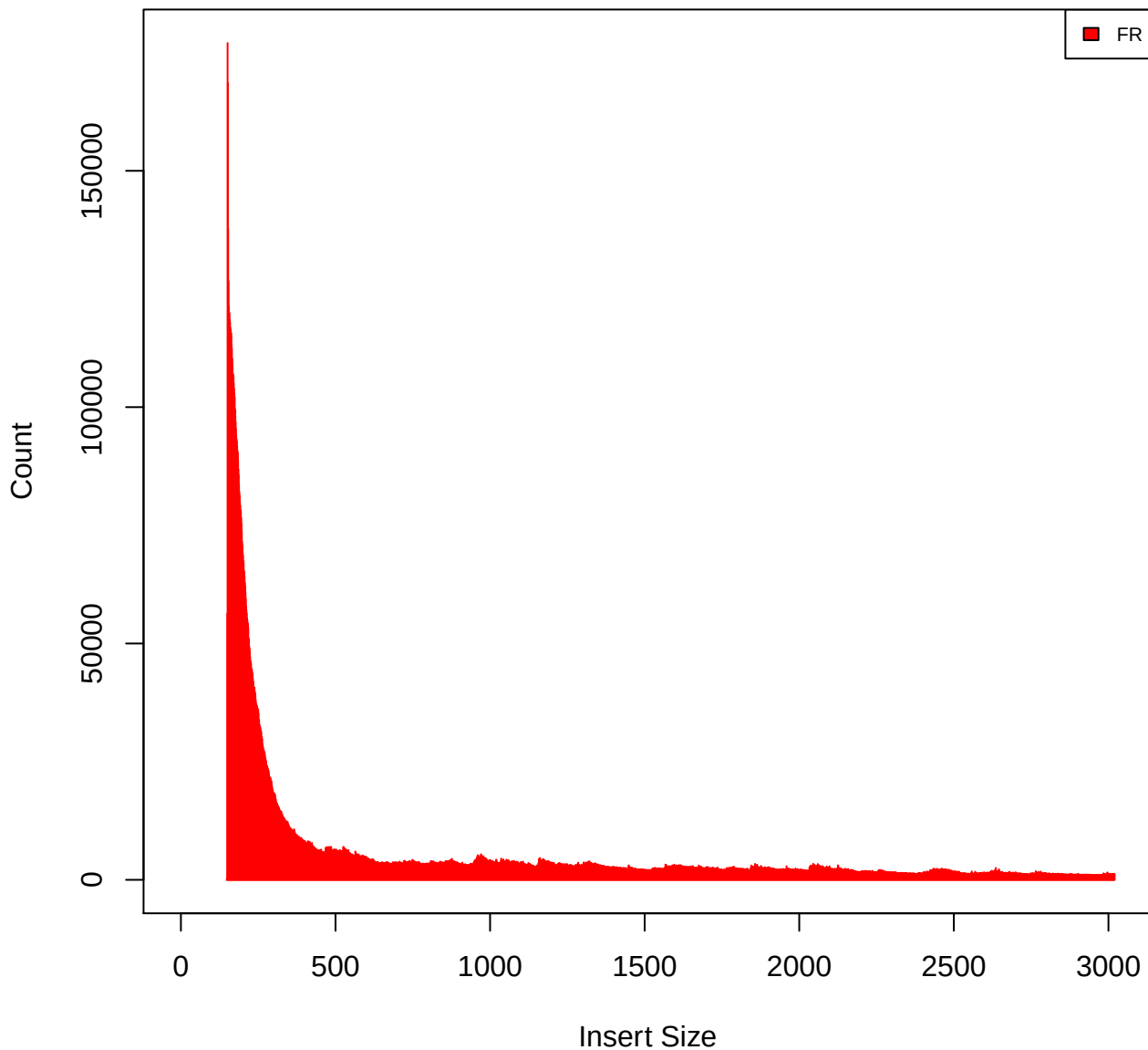
Insert Size Histogram for All_Reads in file G168_G169_M15_primary_unique.bam
