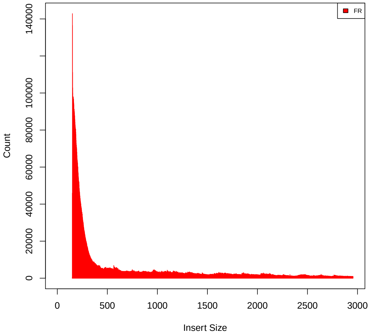
Insert Size Histogram for All_Reads in file G168_G169_M5_primary_unique.bam
