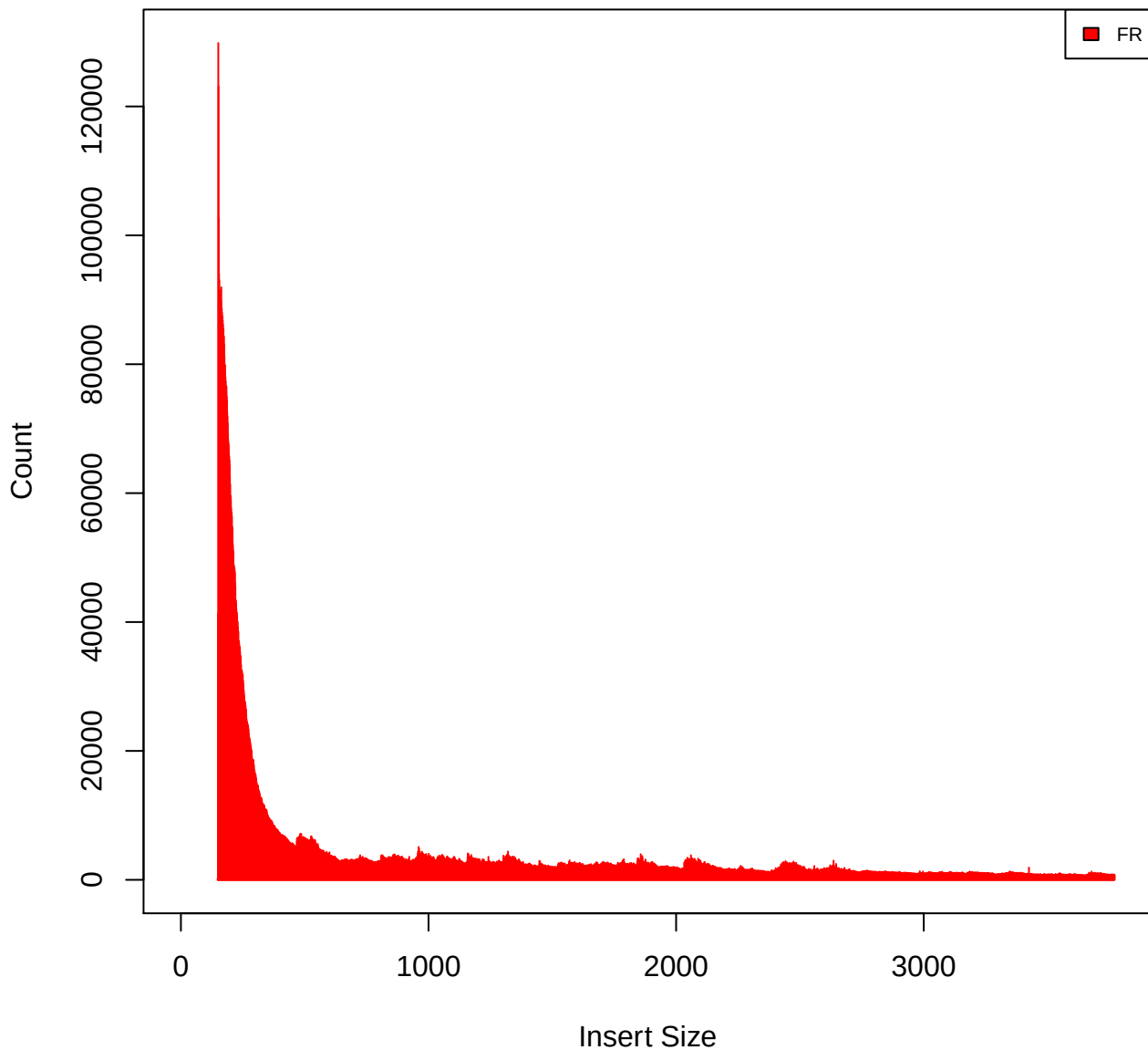
Insert Size Histogram for All_Reads in file G168_G169_M3_primary_unique.bam
