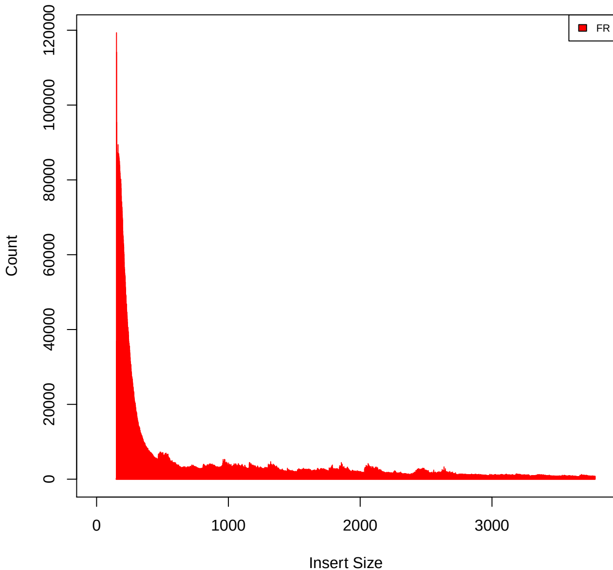
Insert Size Histogram for All_Reads in file G168_G169_M2_primary_unique.bam
