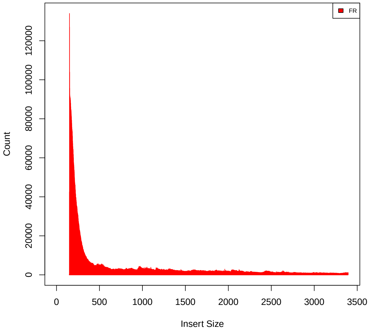
Insert Size Histogram for All_Reads in file G168_G169_M20_primary_unique.bam
