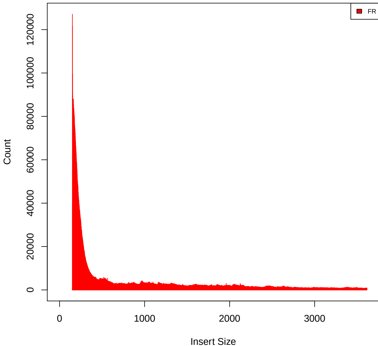
Insert Size Histogram for All_Reads in file G168_G169_M19_primary_unique.bam
