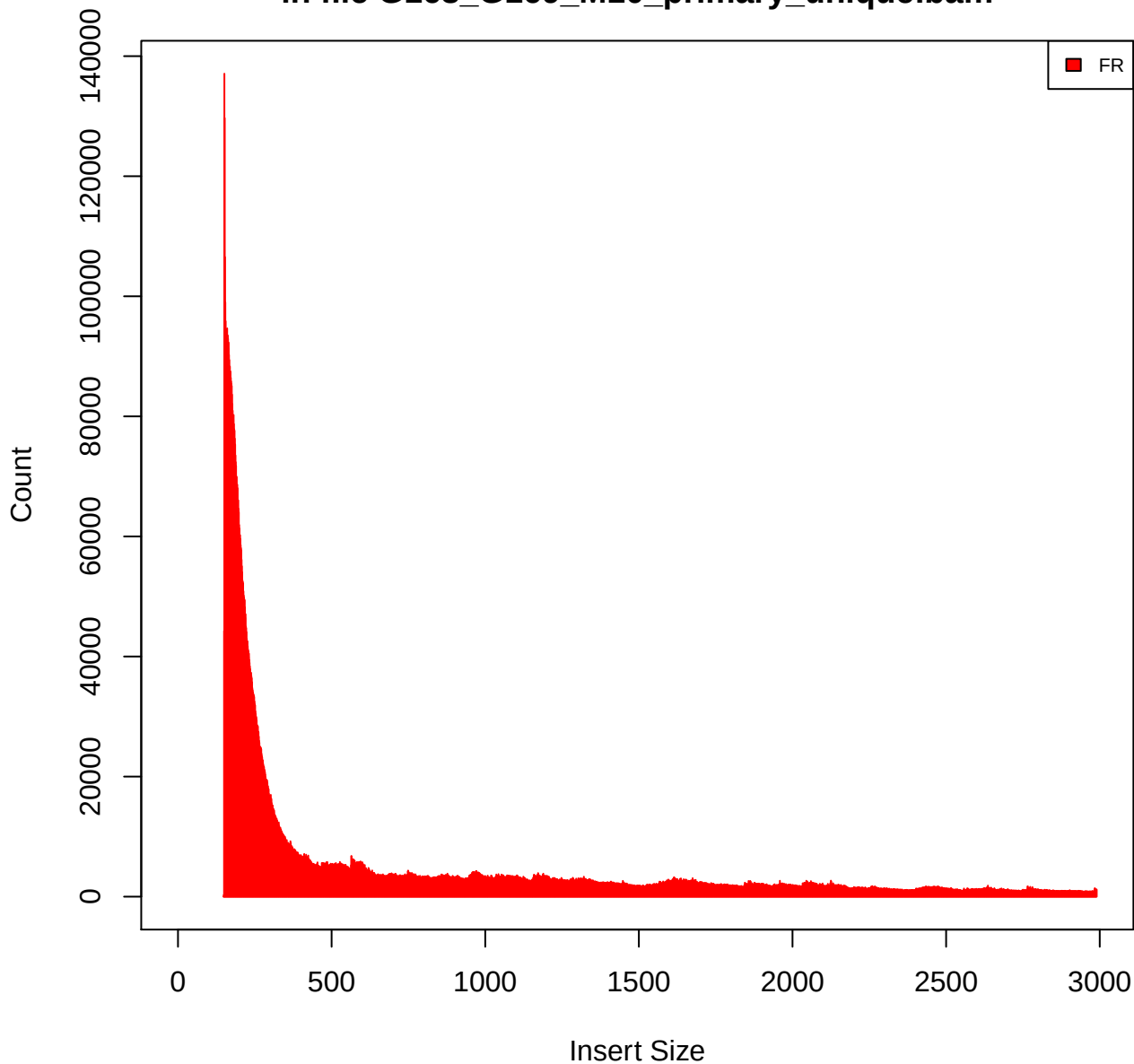
Insert Size Histogram for All_Reads in file G168_G169_M10_primary_unique.bam
