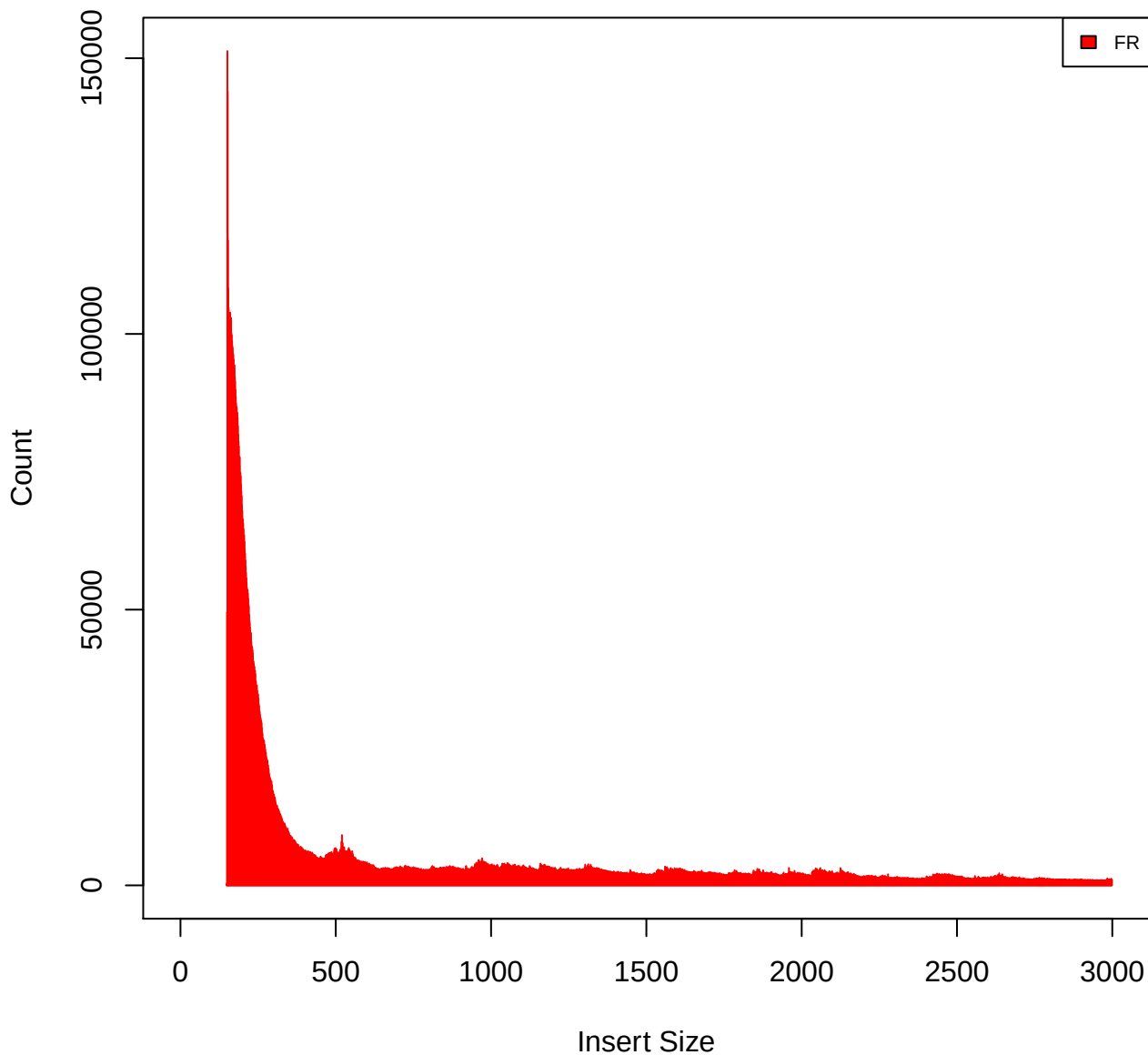
Insert Size Histogram for All_Reads in file G168_G169_M8_primary_unique.bam
