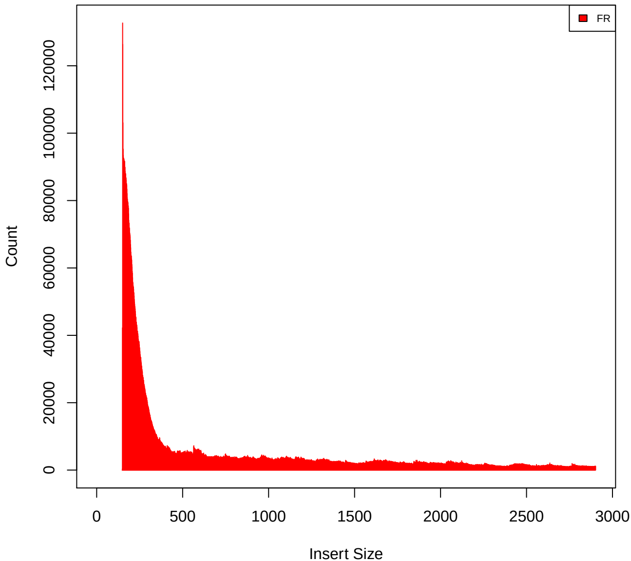
Insert Size Histogram for All_Reads in file G168_G169_M6_primary_unique.bam
