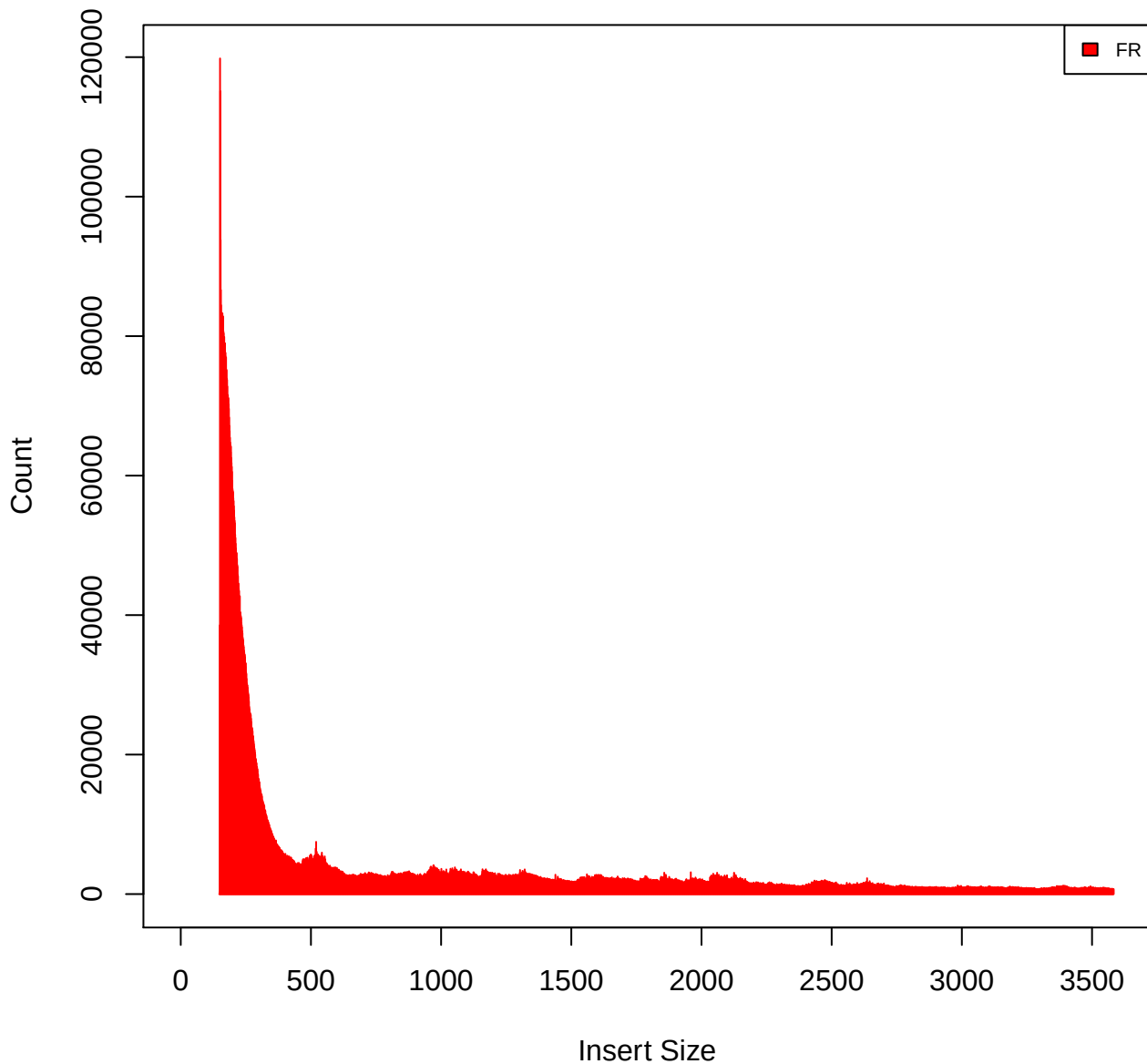
Insert Size Histogram for All_Reads in file G168_G169_M7_primary_unique.bam
