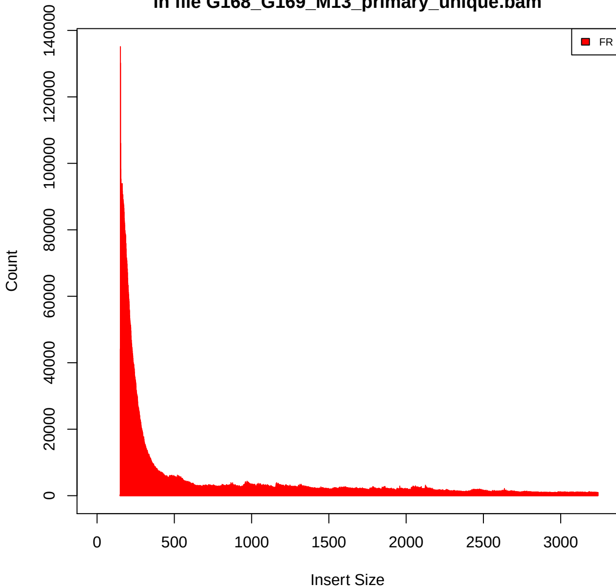
Insert Size Histogram for All_Reads in file G168_G169_M13_primary_unique.bam
