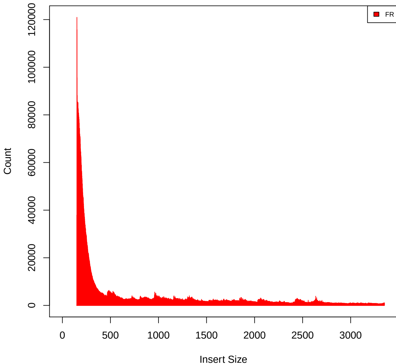
Insert Size Histogram for All_Reads in file G168_G169_M9_primary_unique.bam
