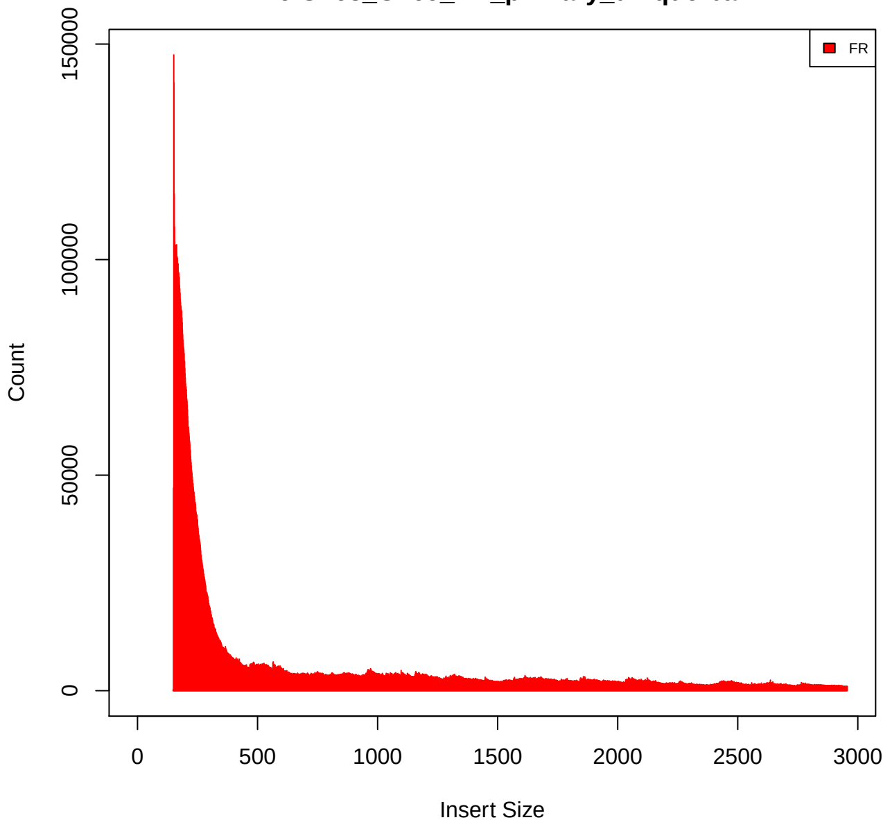
Insert Size Histogram for All_Reads in file G168_G169_M4_primary_unique.bam
