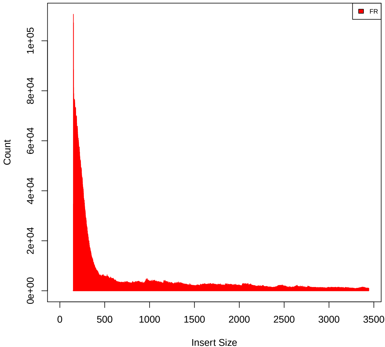
Insert Size Histogram for All_Reads in file G168_G169_M16_primary_unique.bam
