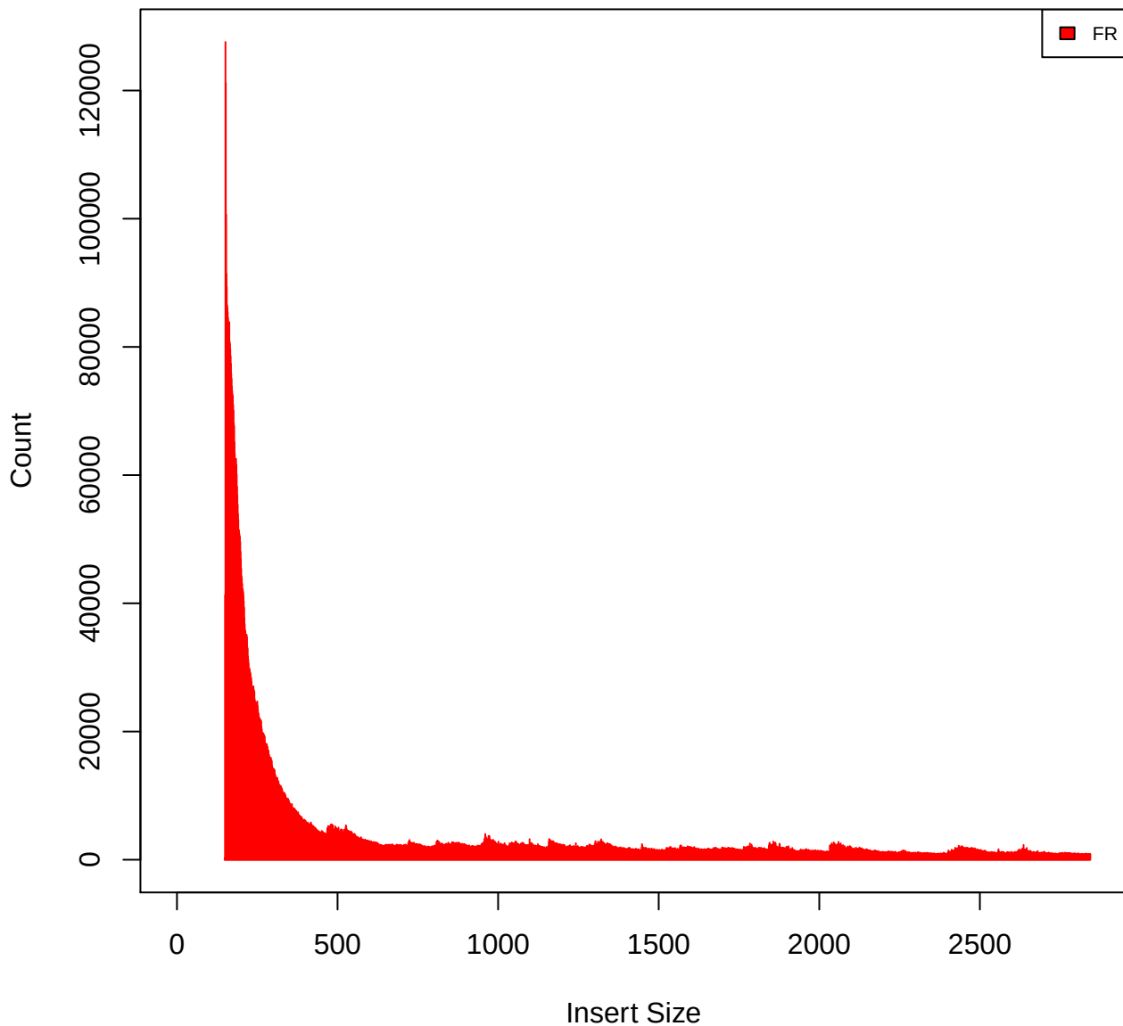
Insert Size Histogram for All_Reads in file G168_G169_M1_primary_unique.bam
